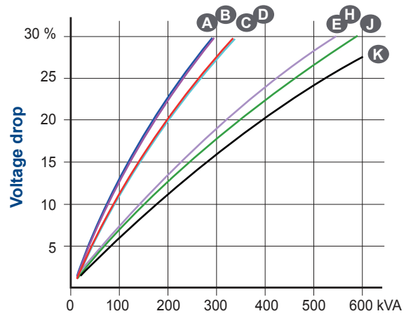
Phase loading (AREP) - kVA at P.F. = 0.8
