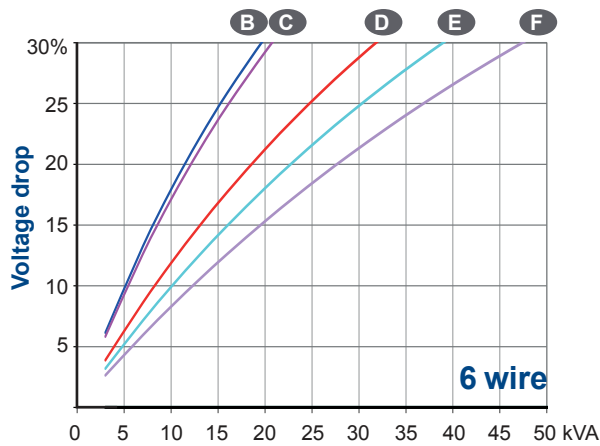
Phase loading (SHUNT/AREP) - kVA at P.F. = 0.8
