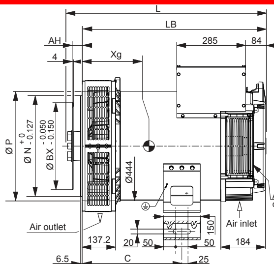
Dimensions (mm) and weight
