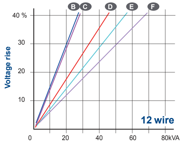
Load shedding (SHUNT/AREP) - kVA at P.F. = 0.8
