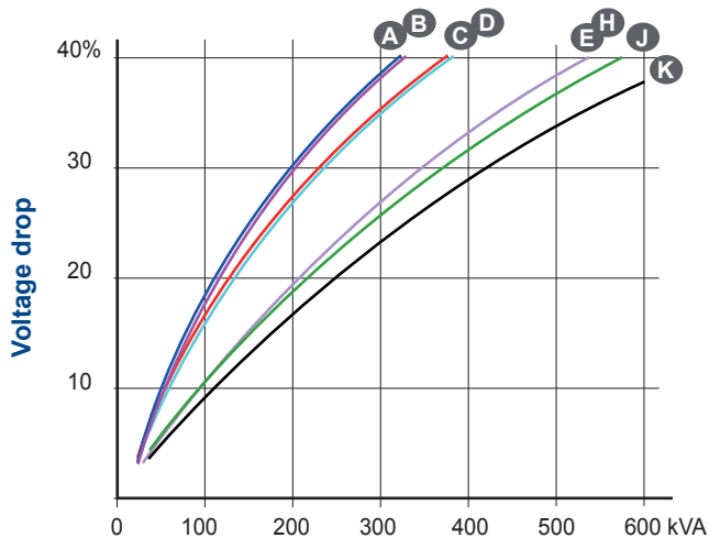
Motor starting (SHUNT) - locked rotor kVA at P.F. = 0.6
