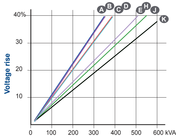
Load shedding (AREP) - kVA at P.F. = 0.8
